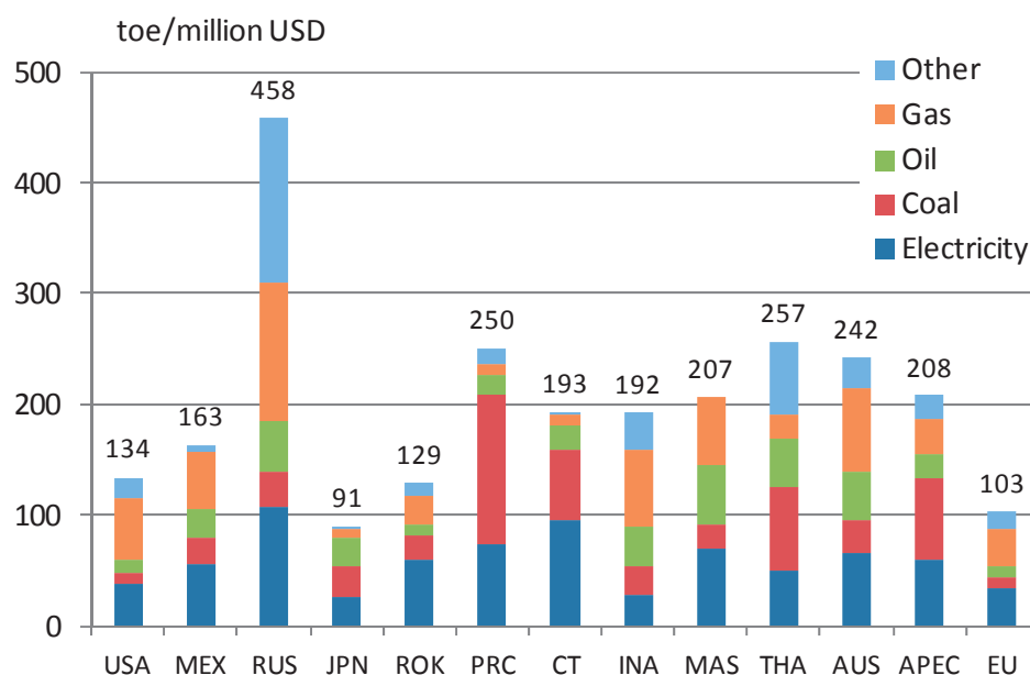
Figure 3-2-1 Final energy consumption per gross value added in manufacturing (2013)
