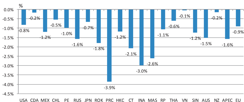
Figure 6-4-2 Change rate of electricity price in the High Efficiency case
